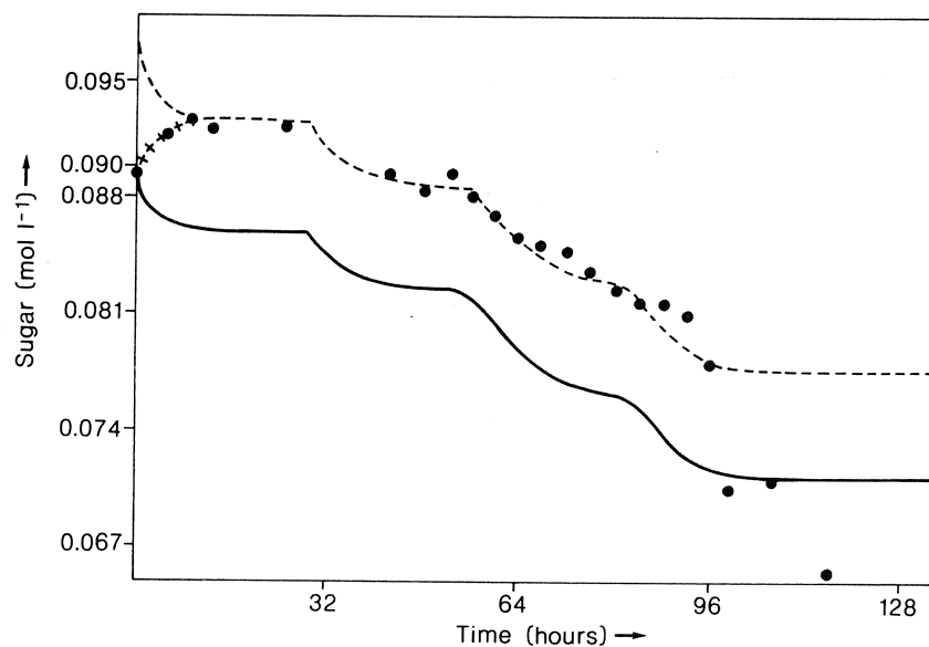
Fig.6.4. Concentration of total sugar in the medium during the first 116 h of the experiment ( •••••••••• ). The solid curve represents the concentration of substrate as predicted by the model with the same parameter values as in Fig.6.2.; the dashed curve was obtained by translation of this theoretical curve over plus 6.5 \cdot 10^{-3} \text{ M} .
